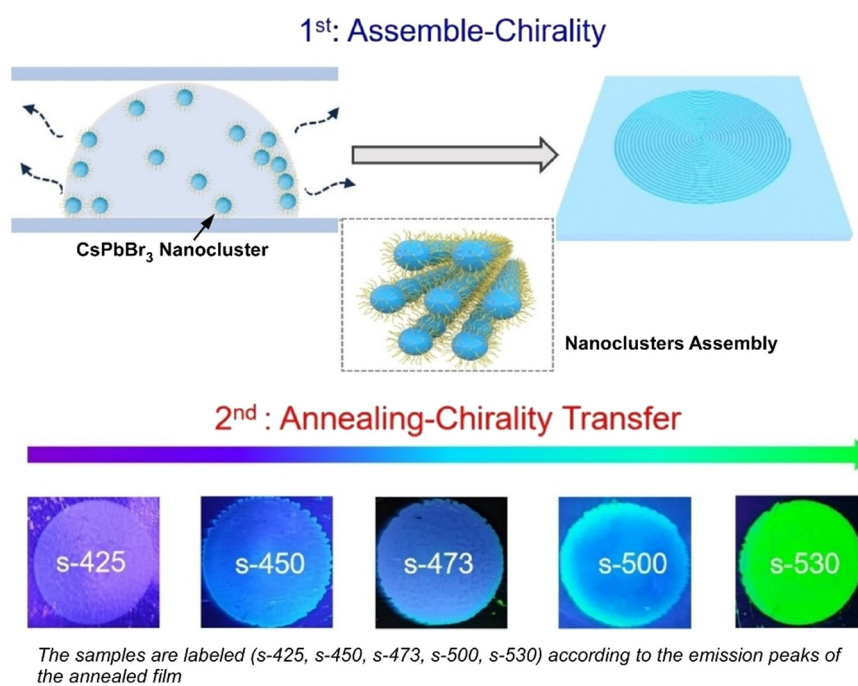
Fig. 24 Fabrication of \text{CsPbBr}_3 superstructures with circularly polarised photoluminescence using a two-step process involving self-assembly of nanoclusters (top) followed by annealing (bottom). Reprinted with permission from ref. 80 copyright 2025 Wiley-VCH.
