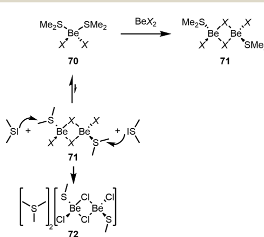
Scheme 15 Nucleophilic attack of non-coordinated \text{SMe}_2 at 71 during the formation of trimethylsulfonium salt 72 . 112
