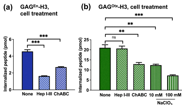
Fig. 4 MALDI-TOF MS quantification of internalized (pmol) chimeric peptides incubated (7 \mu\text{M} ) 1 h at 37 ^{\circ}\text{C} with one million SKOV-3 cells submitted to GAG hydrolysis (HepI-III, ChABC) or desulfation ( \text{NaClO}_3 ).
