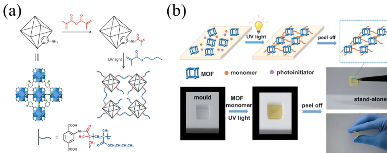
Fig. 1 (a) Functionalization of UiO-66-NH 2 with methacrylic anhydride and polymerization with butyl methacrylate under UV light. (b) Schematic illustration of the formation of MMM via a light-induced grafting-from strategy. Copyright 2015 John Wiley and Sons.
