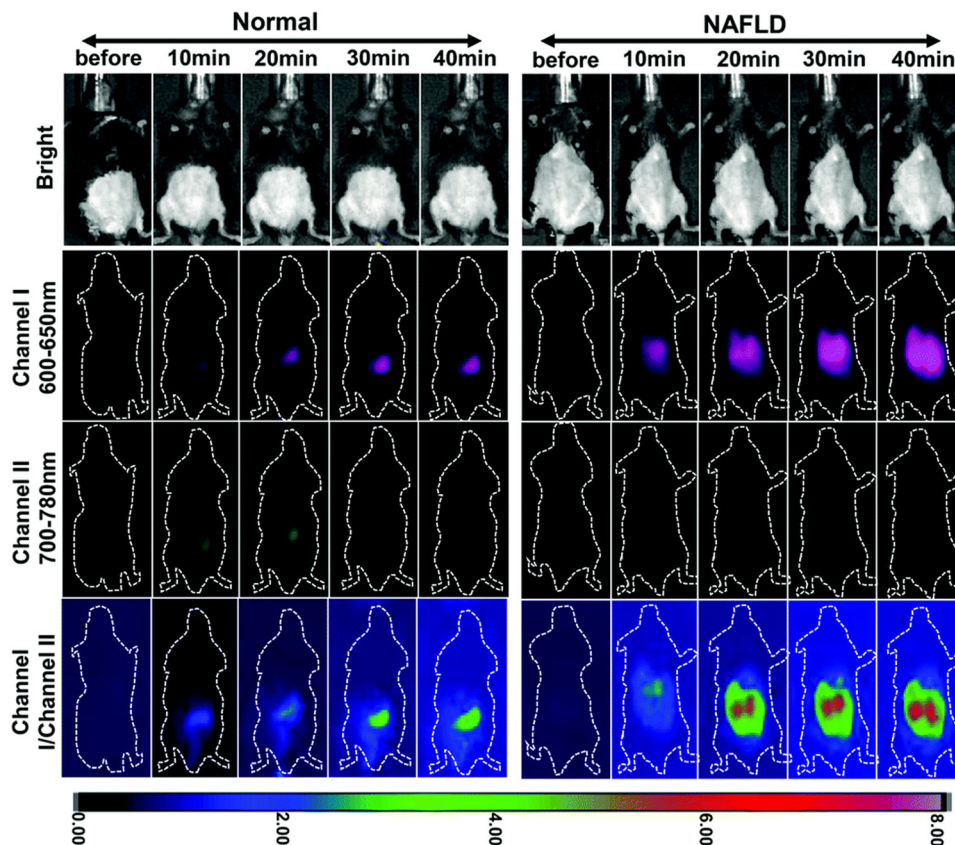
Fig. 20 The ratiometric imaging of normal and NAFLD-bearing mouse models with probe 24 through channel I (600–650 nm), channel II (700–780 nm) and ratio channel (channel I/channel II). Adapted with permission from ref. 133. Copyright 2022 Royal Society of Chemistry.
