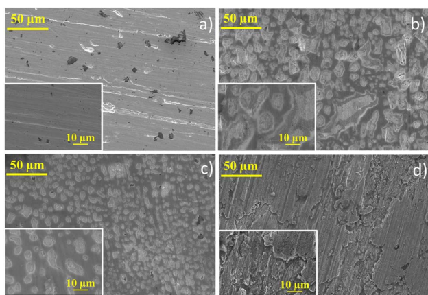
Fig. 3 Scanning electron microscopy images for (a) cleaned Pb plate before the reaction and for the Pb plate after the reaction using (b) acidic anolyte (H 2 SO 4 ), (c) near-neutral anolyte (KHCO 3 ), and (d) alkaline anolyte (KOH).
