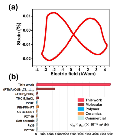
Fig. 2 Piezoelectric properties of 1 . (a) S – E curves of 1 . (b) d_{33} \times g_{33} of 1 compared with those of other reported piezoelectric materials.
