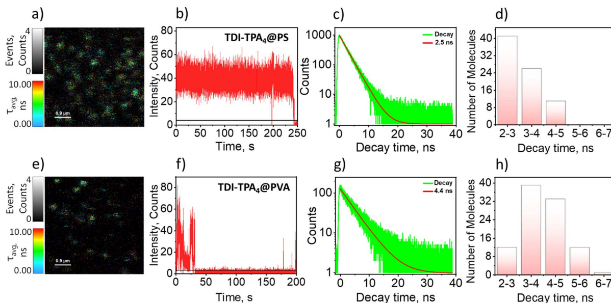
Fig. 3 Representative fluorescence lifetime images with average lifetime ( \tau_{avg} ) and events scale, of TDI-TPA 4 in (a) PS and (e) PVA matrices. Fluorescence intensity trajectories (FITs) of TDI-TPA 4 in (b) PS and (f) PVA matrices. Representative single-molecule fluorescence decay measurements of TDI-TPA 4 in (c) PS and (g) PVA matrices. Fluorescence lifetime distribution plot of TDI-TPA 4 in (d) PS and (h) PVA matrices.
