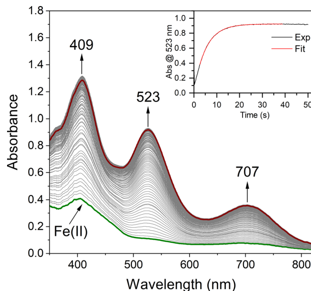
Fig. 1 Time-resolved spectral changes obtained upon mixing THF solutions of five-coordinate [\text{Fe}^{\text{II}}(\text{S}_2^{\text{Me}_2}\text{N}_3(\text{Pr},\text{Pr}))] ( 1 , 0.25 mM) and O 2 (3.95 mM) at -40\text{ }^\circ\text{C} . Inset: kinetic trace ( \lambda = 523\text{ nm} ) showing the formation of the \text{Fe}-\text{O}_2 intermediate 2 . All reported concentrations are after mixing in the stopped-flow cell.
