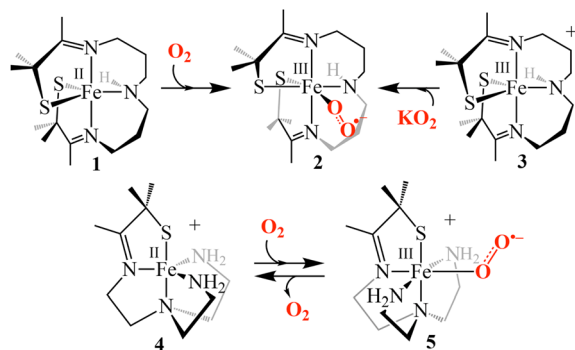
Scheme 1 Pathways for the formation of [\text{Fe}^{\text{III}}(\text{S}_2^{\text{Me}_2}\text{N}_3(\text{Pr},\text{Pr}))(\text{O}_2)] ( 2 ) (top), and reversible dioxygen binding to [\text{Fe}^{\text{II}}(\text{S}^{\text{Me}_2}\text{N}_4(\text{tren}))]^+ ( 4 ) to form a putative superoxo intermediate [\text{Fe}^{\text{III}}(\text{S}^{\text{Me}_2}\text{N}_4(\text{tren}))(\text{O}_2)]^+ ( 5 ) (bottom).
