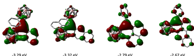
Fig. 6 LUMO images of 1–4 (from left to right, isovalue: \pm 0.03 ).
