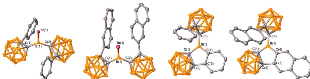
Fig. 3 Solid-state structures of \text{BrB}^{\text{Ph}}\text{oCb}_2 , \text{BrB}^{\text{2Np}}\text{oCb}_2 , 1 , and 2 (from left to right). Hydrogen atoms are omitted for clarity and thermal ellipsoids are drawn at the 50% probability level.
