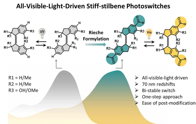
Fig. 1 Molecular structures of the stiff-stilbenes S1 – S6 controlled using UV light and visible light, respectively, and cartoon representation of the absorption band of stiff-stilbenes substituted with aldehydes ( S2 , S4 , and S6 ) and those without formyl group ( S1 , S3 , and S5 ).
