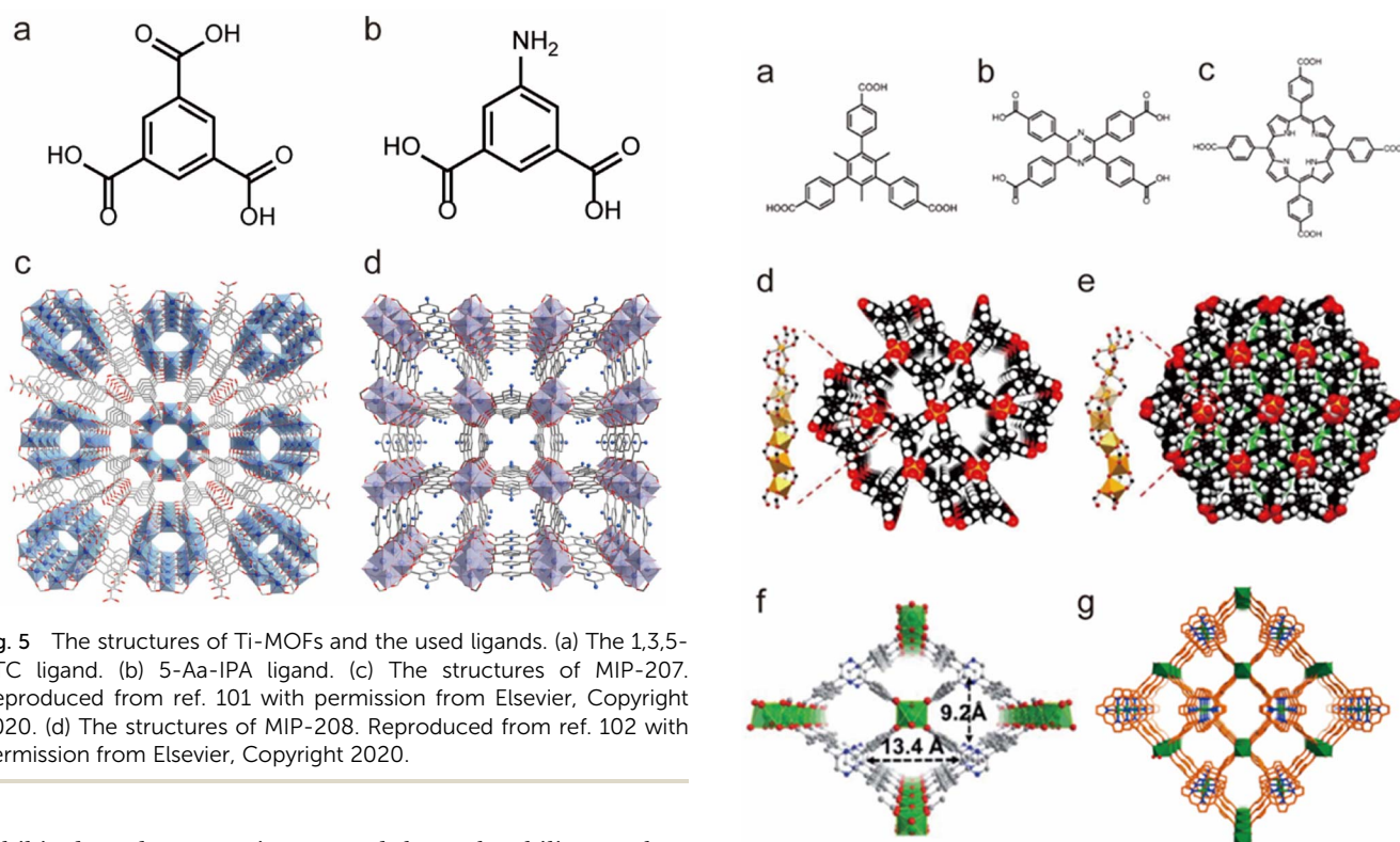
Fig. 6 The structures of representative In(III)-MOFs and the used ligands. (a) The H_3CTTA ligand. (b) The H_4TCP ligand. (c) The H_2TCP ligand. (d) BUT-172. Reproduced from ref. 103 with permission from the Royal Society of Chemistry, Copyright 2020. (e) BUT-173. Reproduced from ref. 103 with permission from the Royal Society of Chemistry, Copyright 2020. (f) In(tcp). Reproduced from ref. 104 with permission from the Royal Society of Chemistry, Copyright 2021. (g) USTC-8. Reproduced from ref. 105 with permission from the American Chemical Society, Copyright 2018.
