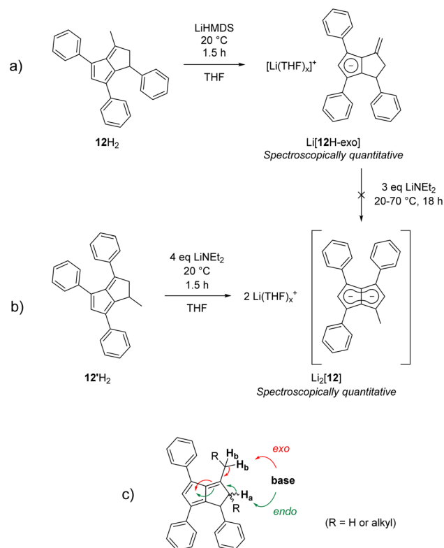
Scheme 7 (a) Exocyclic deprotonation of 12 H 2 to Li[ 12 H-exo] with LiHMDS; (b) formation of Li 2 [ 12 ] from 12 'H 2 with LiNEt 2 ; (c) allylic deprotonation competition in 3-alkylated dihydropentalenes.
