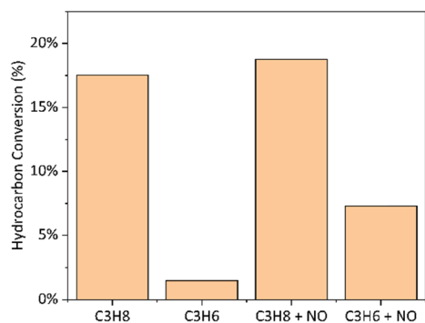
Fig. 2 Comparison of conversion of C 3 H 8 and C 3 H 6 over hBN in the presence/absence of NO. Conditions: 550 °C, 7 mm tube, ~30% C 3 H 8 or C 3 H 6 /15% O 2 /0 or 150 ppm NO/~55% N 2 , 40 mL min -1 total flow, 100 mg hBN diluted in 500 mg SiC.
