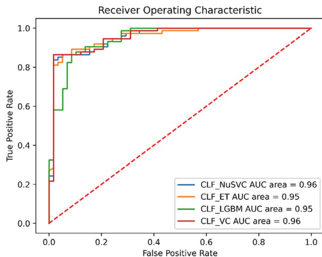
Fig. 3 ROC curve of the individual classifiers and voting classifier.
