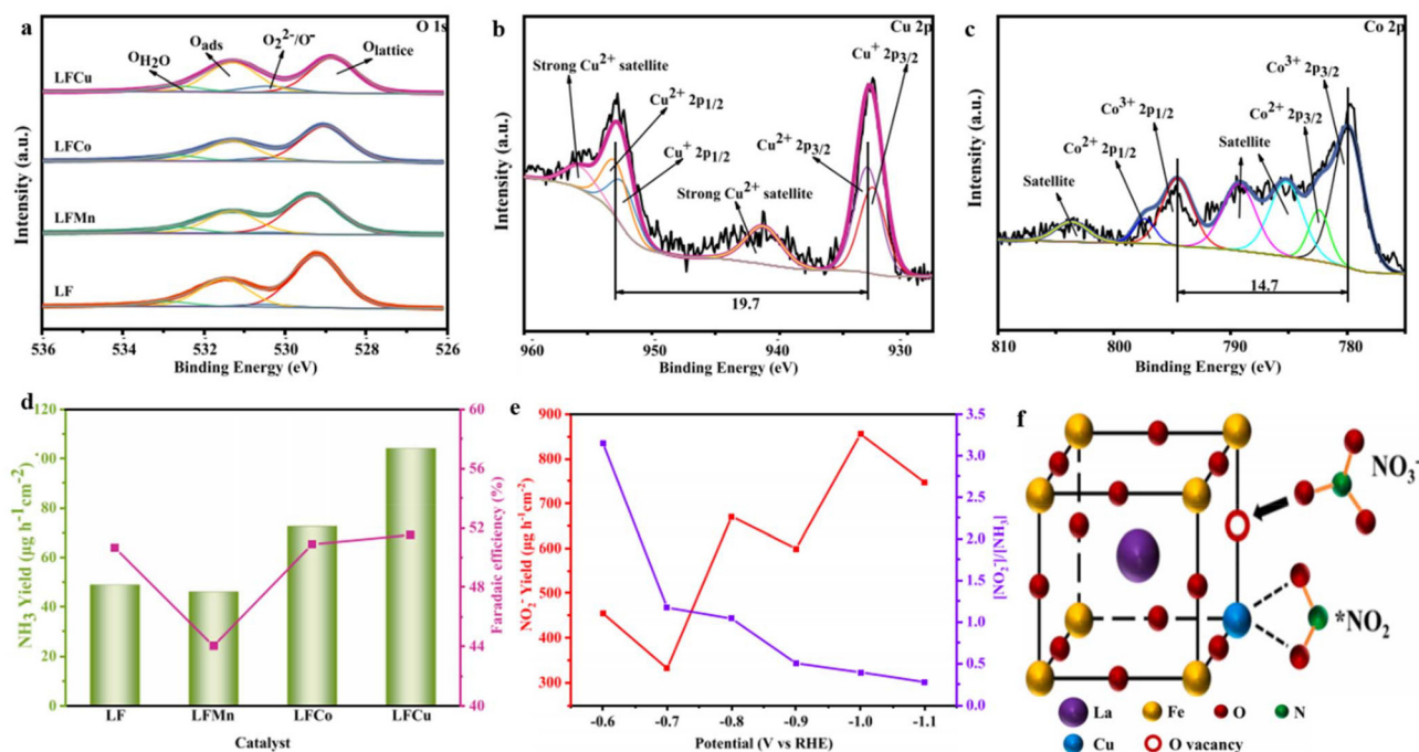
Fig. 15 (a–c) XPS spectra of O 1s, Cu 2p of LFCu, and Co 2p of LFCo. (d) Yield rate and \text{Fes}(\text{NH}_3) of the respective catalysts at -0.7 V (vs. RHE). (e) \text{NO}_2^- production and the ratio of [\text{NO}_2^-] to [\text{NH}_3] on LFCu at various potentials, (f) schematic representation of \text{NO}_3^- reduction on LFCu. Reproduced from ref. 195 with permission from Elsevier, copyright 2023.
