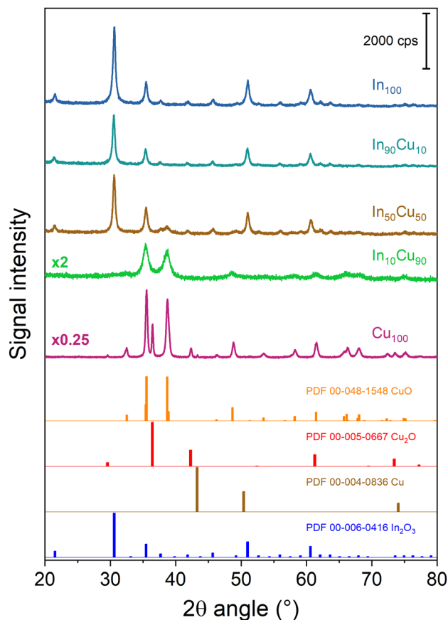
Fig. 3 XRD diffractograms of the fresh calcined samples. For the sake of clarity, a diffractogram with multiplicative values has the measured intensity multiplied by that factor.
