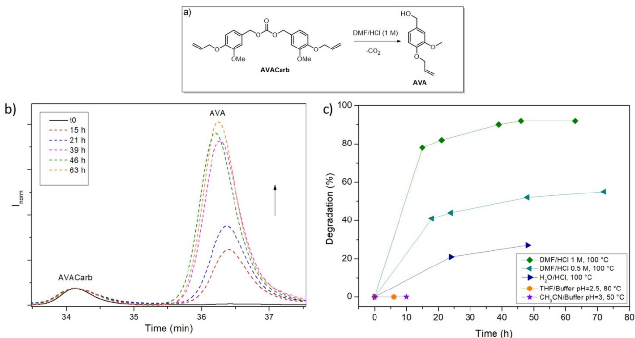
Fig. 6 (a) Molecular model: cleavage of AVACarb into AVA under acidic conditions, (b) monitoring of the degradation in DMF/HCl 1 M at 100 ^\circ\text{C} via SEC, (c) establishment of degradation conditions for AVACarb : test of different reaction conditions.
