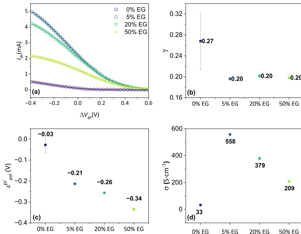
Fig. 6 (a) Transfer curves (hollow circles) from Rivnay (2016), and fitting curves (solid lines), (b) \gamma , (c) E_{pol}^0 and (d) \sigma parameters. Reprinted (adapted) with permission from Rivnay et al. (2016). 47 For all adjustments R^2 = 0.99 and p -values < 0.05 .
