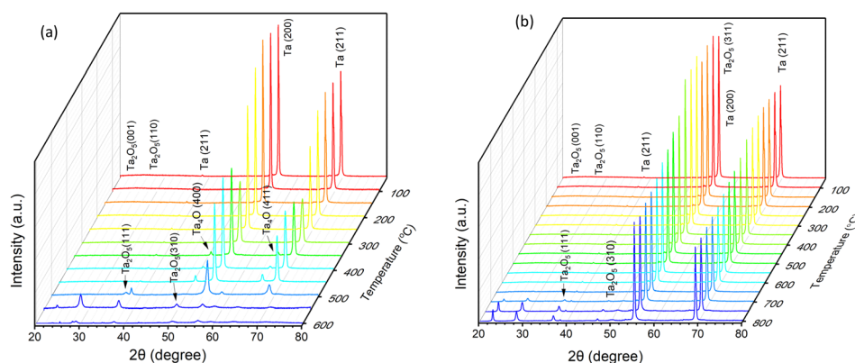
Fig. 10 Temperature programmed XRD spectra under an (a) air and (b) argon atmosphere for ATO structures formed at the applied potential of 30 V for 4 min in the electrolyte containing 90 ml \text{H}_2\text{SO}_4 (95 wt%) + 6 ml of HF (40 wt%) + 4 ml \text{H}_2\text{O} .
