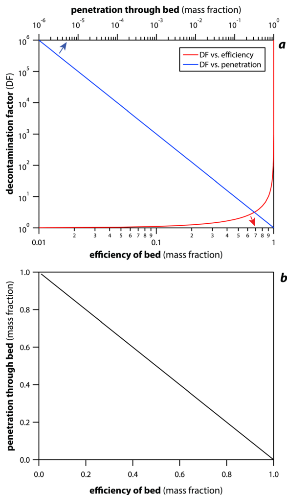
Fig. 15 Summary showing the relationships between DF, bed efficiency (to 0.999999), and bed penetration (to 0.000001), including (a) DF vs. both bed efficiency and bed penetration (all axes are log 10 ) as well as (b) bed penetration vs. bed efficiency.
