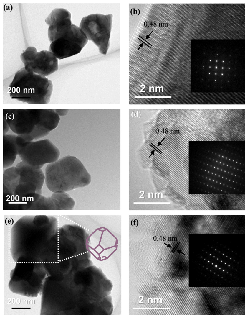
Fig. 4 HR-TEM images of (a) and (b) LMO, (c) and (d) LMTOS, and (e) and (f) LMTOS (scale bar: 200 nm and 2 nm), and the inset shows the corresponding SAED pattern (region shown in (b) LMO, (d) LMTOS and (f) LMTOS particles).
