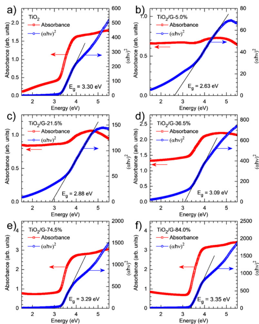
Fig. 23 UV-vis diffuse reflectance spectra and related Tauc plots of TiO 2 (a) and TiO 2 /graphene with varying TiO 2 loadings (5% (b), 21.5 (c), 36.5% (d), 74.5% (e), and 84% (f)). Reprinted with permission from ref. 131 Copyright 2021, Elsevier.
