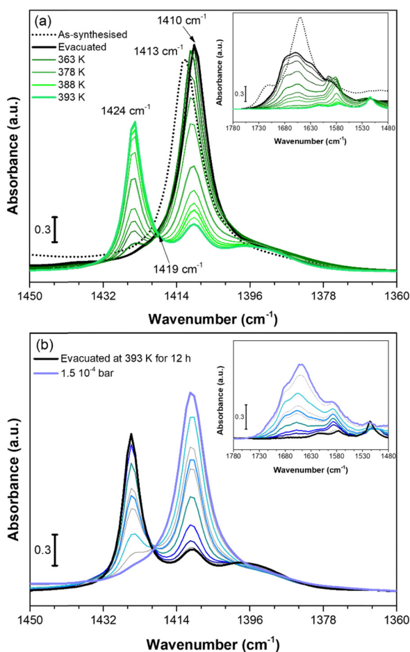
Fig. 6 IR spectra of Cu-EtP collected in the 313\text{--}393 \text{ K} temperature range (a) and dosing 0.35\text{--}1.5 \times 10^{-4} \text{ bar} of \text{H}_2\text{O} (b), reported in the 1450\text{--}1360 \text{ cm}^{-1} spectral region. Dashed black curves represents the as synthesised Cu-EtP, black curves the evacuated sample at RT (a) and 393 \text{ K} (b), green bold curves represent Cu-EtP spectra at increasing temperatures and blue bold curves the incremental pressure doses of \text{H}_2\text{O} employed during the IR experiment and specified in Fig. S41 (ESI†). The insets report the corresponding 1780\text{--}1480 \text{ cm}^{-1} spectral region.
