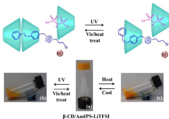
Fig. 47 (a) Mode of inclusion between b-CD and AzoIPS-LiTFSI before and after UV irradiation. (b) Preparation of the supramolecular hydrogel: (a) b-CD/AzoIPS-LiTFSI (3 : 1), and its disassembly induced by: (b) UV light, and (c) temperature. Reproduced from ref. 226 with permission from Wiley-VCH, Copyright [2018].
