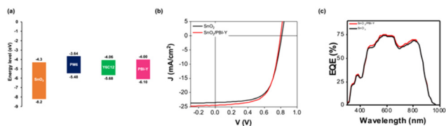
Fig. 5 (a) The energy levels of \text{SnO}_2 , PM6, Y6C12 and PBI-Y. (b) J - V curves and (c) EQE spectra of spin-coated \text{SnO}_2 /PBI-Y devices (red) compared to reference with \text{SnO}_2 only (black).
