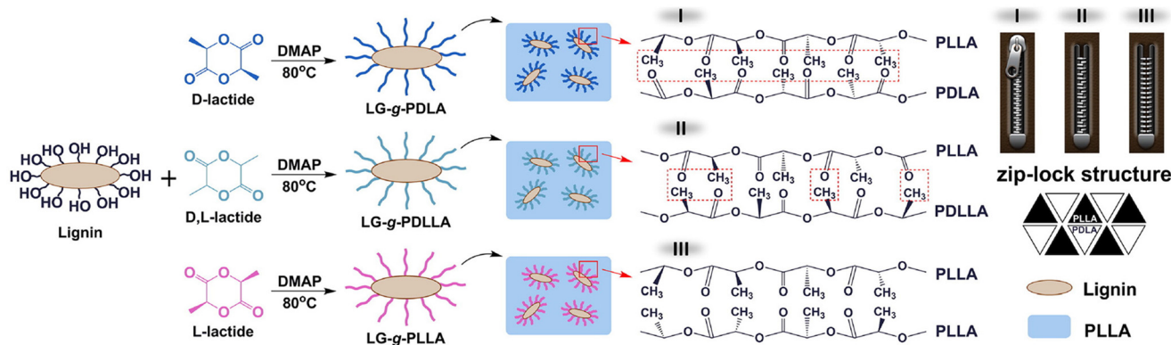
Fig. 12 Illustration of the synthesis of LG-g-PDLA (-PDLA, -PDLA) and structures of the stereocomplex films. Reproduced from ref. 112 with permission from Elsevier, copyright 2017.
