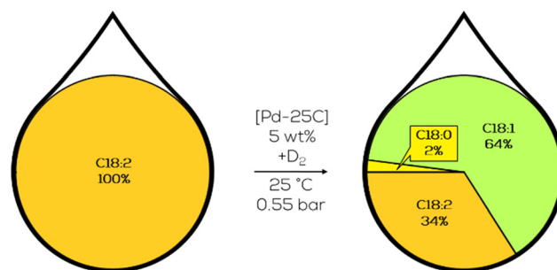
Fig. 17 C18 fatty acid composition in the deuteration of methyl linoleate with Pd on carbon as performed by Koritala et al. 109
