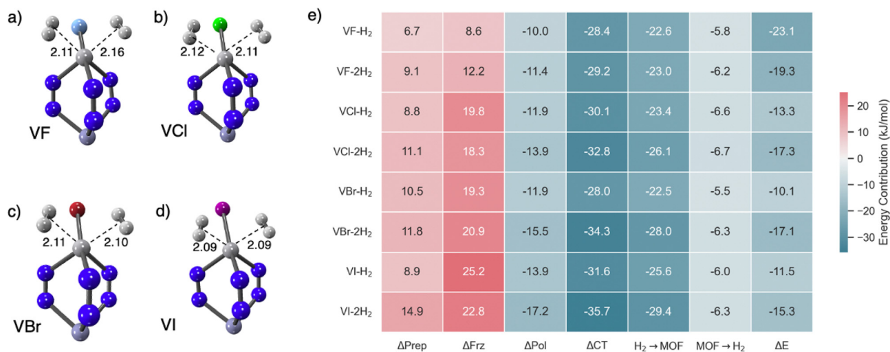
Fig. 13 Multiple H 2 ligations in V(II)-X-MFU-4l, (X = F, Cl, Br, I) (a)–(d) and EDA of the quite wide range of adsorption behaviour as a function of the halide counterion (e). Dative effects, particularly forward donation, dominate the binding energy. Distances are reported in Å, and energy contributions in kJ mol -1 in (e).
