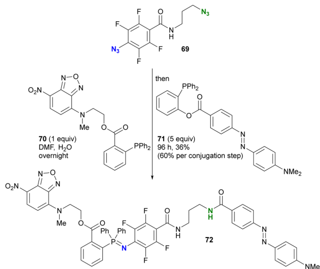
Scheme 13 Azide-site-selective sequential double Staudinger reaction conjugation of aryl- and alkyl-azido-containing diazide.
