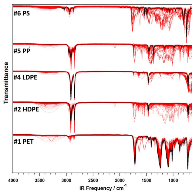
Fig. 2 Mid-infrared ( 4000\text{--}650\text{ cm}^{-1} ) spectra of 835 postconsumer plastics that were evaluated in this study (red). Virgin polymer (black). Spectra are shown in percent transmittance ( y -axis minimum is 30% per RIC).
