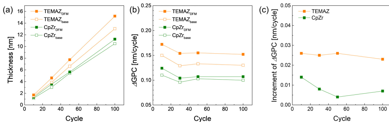
Fig. 2 (a) \text{ZrO}_2 thin film thickness, (b) differential growth rate ( \Delta\text{GPC} ), and (c) increment of growth rate with respect to the cycle number varied by employing precursors and sequence.
