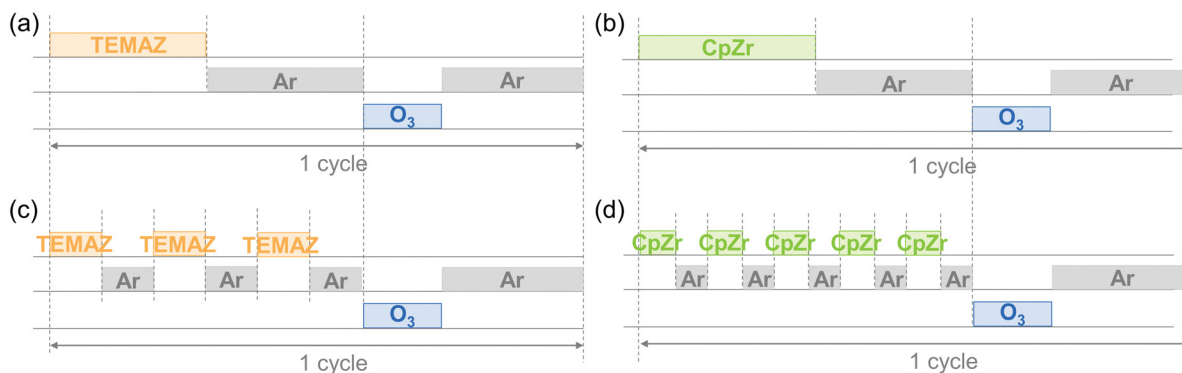
Fig. 1 Schematic of the ALD process sequences of base sequence with (a) TEMAZ ( \text{TEMAZ}_{\text{base}} ), (b) CpZr ( \text{CpZr}_{\text{base}} ), and DFM sequence with (c) TEMAZ ( \text{TEMAZ}_{\text{DFM}} ), (d) CpZr ( \text{CpZr}_{\text{DFM}} ).
