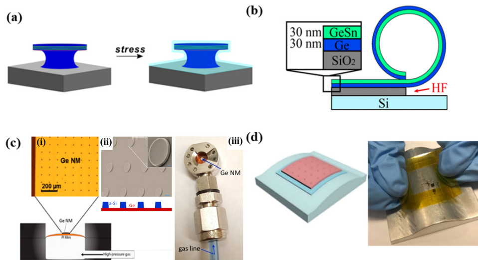
Fig. 4 Various strain-engineering strategies for GeSn NMs: (a) Tensile strained GeSn microdisk using high-stress \text{SiN}_y stessor layer. 58 Reprinted with permission from ref. 58. Copyright 2016, American Chemical Society. (b) A schematic diagram describing the rolling up procedure for the GeSn/Ge bilayer. 59 Reproduced with permission from ref. 59. Copyright 2018, IOP Publishing. (c) (i) Schematic illustration of the experimental setup for biaxial tensile strained Ge NMs, 60 (ii) SEM image with a schematic of a Ge NM coated with an a-Si pillar array, and a photograph of the pressure cell loaded with a Ge NM. 61 Reproduced with permission from ref. 60 and 61. Copyright 2018, 2021, MDPI, American Chemical Society. (d) Schematic structure and optical image of flexible GeSn NMs where uniaxial strains are introduced by placing conformally on bending fixtures. 62 Reproduced with permission from ref. 62. Copyright 2021, IOP Publishing.
