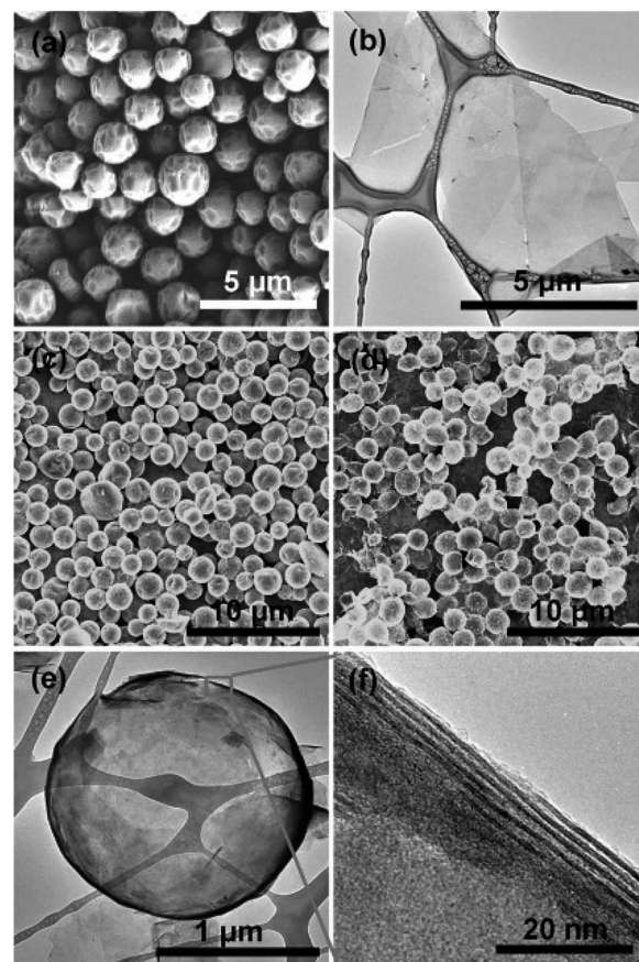
Fig. 5 (a) SEM images showing the morphology of the as-produced PMMA spheres. (b) TEM image of Ti 3 C 2 T x flakes. SEM image of (c) Ti 3 C 2 T x /PMMA hybrids and (d) hollow Ti 3 C 2 T x spheres after removal of PMMA, showing that the spherical shape is retained after PMMA's thermal evaporation at 450 °C. TEM images showing (e) a hollow Ti 3 C 2 T x sphere and (f) its wall MXene layers. Reproduced with permission from ref. 84, Copyright 2017 Wiley Publications.
