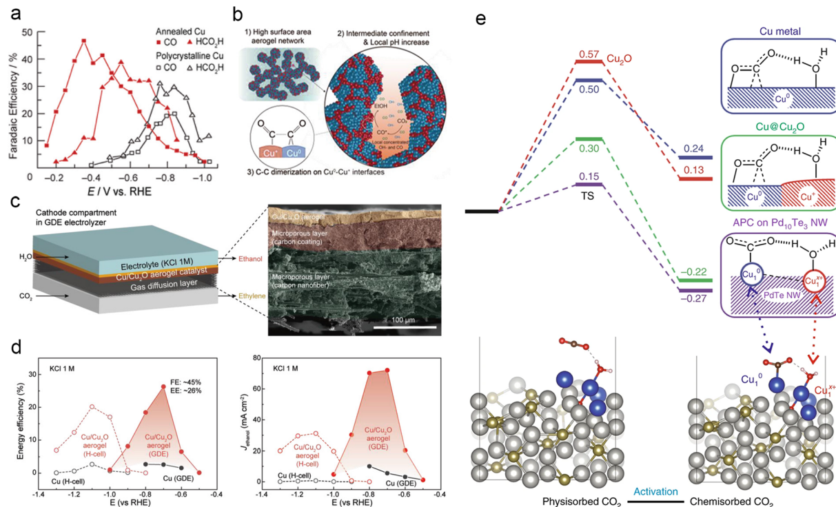
Fig. 10 (a) Product distribution for CO and HCOOH of polycrystalline Cu and Cu annealed at 500 °C for 12 h (resulting in \text{Cu}_2\text{O} layers). Reproduced from ref. 185. Copyright 2012 American Chemical Society. (b) Schematic representation of the mechanism promoting ethanol production on \text{Cu/Cu}_2\text{O} aerogels and proposed origin. (c) Schematic diagram of the flow cell reactor and cross-sectional SEM images of the \text{Cu/Cu}_2\text{O} aerogel on the GDE. (d) Comparison of \text{EE}_{\text{EtOH}} and J_{\text{EtOH}} for \text{Cu/Cu}_2\text{O} aerogels and Cu films in H-cell and flow-cell reactors, respectively. Reproduced from ref. 187. Copyright 2021 Wiley-VCH. (e) Free energy curves of \text{CO}_2 activation on Cu, \text{Cu@Cu}_2\text{O} and APCs of \text{Cu}_{10}\text{-Cu}_1^{x+} on \text{Pd}_{10}\text{Te}_3 nanowires, respectively (at -0.78 V vs. RHE) (above). Conformations of physisorbed and chemisorbed \text{CO}_2 on Cu-APC (below). Reproduced from ref. 188. Copyright 2019 Nature.
