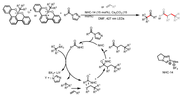
Scheme 28 Synthesis of ketones from alkylborates and alkyl acyl imidazoles.
