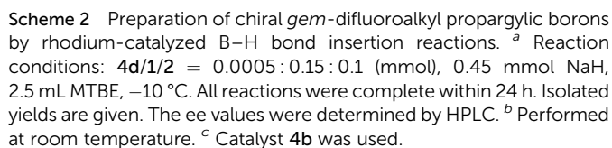
with an electron-donating methyl group or an electron-withdrawing fluorine or chlorine atom or a trifluoromethyl group on the 1-phenyl ring were tolerated ( 3ja–3qa ). Compounds with a 1-naphthyl or 1-thienyl group attached to the alkynyl moiety showed high yields and enantioselectivities ( 3ra, 3sa ). When 4b was the catalyst, a substrate with a methyl group attached to the gem -difluoromethylene group afforded 3ta in good yield with moderate enantioselectivity. We also evaluated reactions of 1a with a series of borane adducts 2 and found that only trialkylamine–borane adducts afforded good results (see the ESI† for details). The structure and absolute configuration of ( R )- 3fa were determined by X-ray diffraction analysis of a single crystal.
