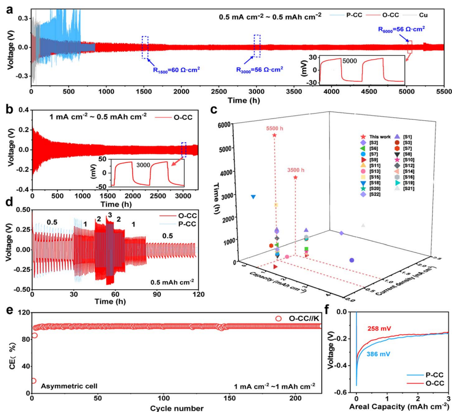
Fig. 2 Electrochemical performance. Galvanostatic cycling performance of P-CC and O-CC in symmetric cells at (a) 0.5 \text{ mA cm}^{-2} and (b) 1 \text{ mA cm}^{-2} ; (c) comparison of all the host materials' performance for the K metal anode in symmetric cells; (d) cycling performance of P-CC and O-CC in symmetric cells at different current densities with the areal capacity of 0.5 \text{ mA h cm}^{-2} ; (e) CE curves for O-CC//K asymmetric cells at 1 \text{ mA cm}^{-2}/1 \text{ mA h cm}^{-2} ; (f) nucleation overpotential of P-CC and O-CC at 0.5 \text{ mA cm}^{-2} .
