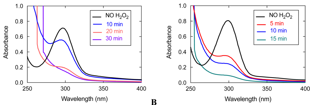
Fig. 5 UV/vis spectra of reactions between 3 and \text{H}_2\text{O}_2 . (A) Data for the reaction between 0.1 mM 3 and 10 mM \text{H}_2\text{O}_2 . (B) Data for the reaction between 0.1 mM 3 and 0.60 mM \text{H}_2\text{O}_2 . All data were taken in 50 mM HEPES buffered to pH 7.00 at 298 K with a 1.0 cm cuvette.
