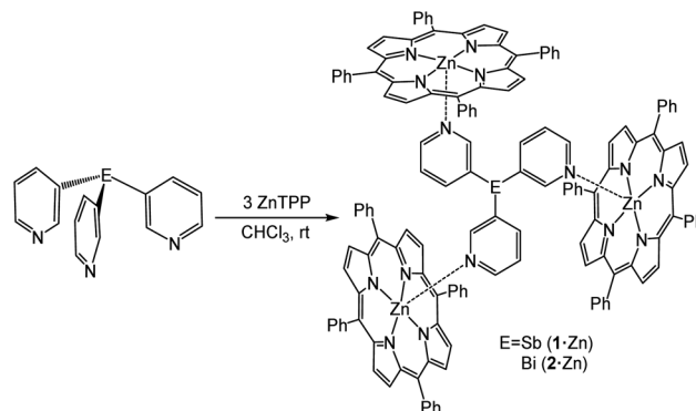
Scheme 1 Synthesis of the capsules {[Sb(3-py) 3 ]·(ZnTPP) 3 } (1·Zn) and {[Bi(3-py) 3 ]·(ZnTPP) 3 } (2·Zn).
