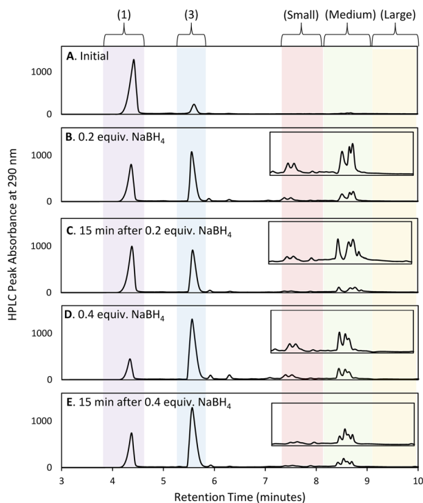
Fig. 9 Chromatograms for synthesis of 4 via dose-wise addition of \text{NaBH}_4 with regional analysis zones identified and highlighted. Sample taken before the addition of \text{NaBH}_4 (A), immediately following first addition of 0.2 equiv. \text{NaBH}_4 (B), and 15 min after \text{NaBH}_4 (C), additional 0.2 equiv. \text{NaBH}_4 (0.4 equiv. cumulative total) (D) and 15 min delay (E).
