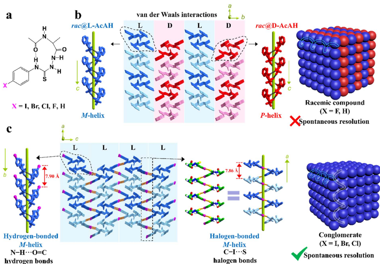
Fig. 6 (a) Chemical structures of AcAX. (b) Heterochiral 2D layers constructed by only N-H\cdots O=C hydrogen bonds and weak van der Waals interactions, which further forms 3D racemic compounds ( X = F and H ). (c) Homochiral 2D layers constructed by both N-H\cdots O=C hydrogen bonds and C-X\cdots S halogen bonds, which further form 3D conglomerates ( X = I, Br , and Cl ). 169 Reproduced with permission from ref. 169. Copyright 2022, John Wiley and Sons.
