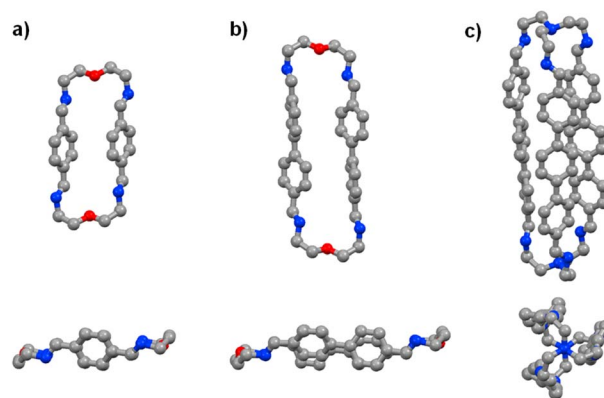
Fig. 1 Single-crystal X-ray structures of the macrocycles pPh 2 (NON) 2 and BiPh 2 (NON) 2 as well as of the macrobicyclic cage TriPh 3 T 2 (side and front/axial views). Colour scheme: carbon (grey), nitrogen (blue), oxygen (red). Hydrogen, H_2O and CHCl_3 molecules are omitted for clarity, see details in ESI, Fig. S63–S65.†
