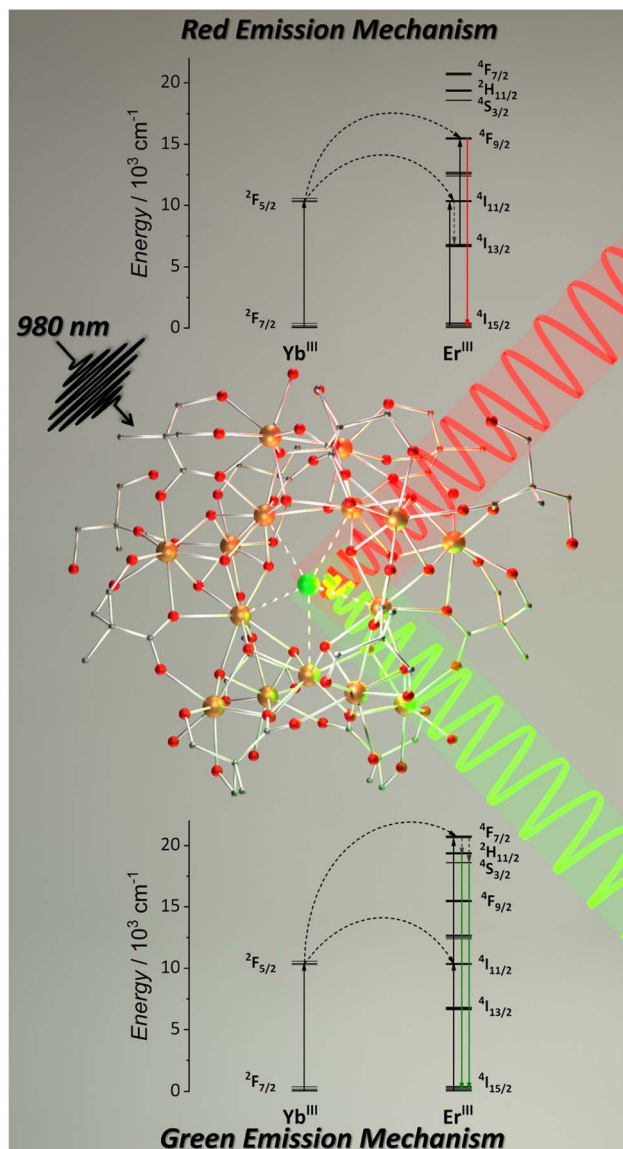
Fig. 6 Single-crystal structure for {Ln 15 } MCAs (CCDC number: 2023378) and mechanism for red and green UC emissions. 92 Colour code: Dark orange: Ln 3+ ; grey: carbon; red: oxygen. Hydrogen atoms were omitted in the structure for clarity.
