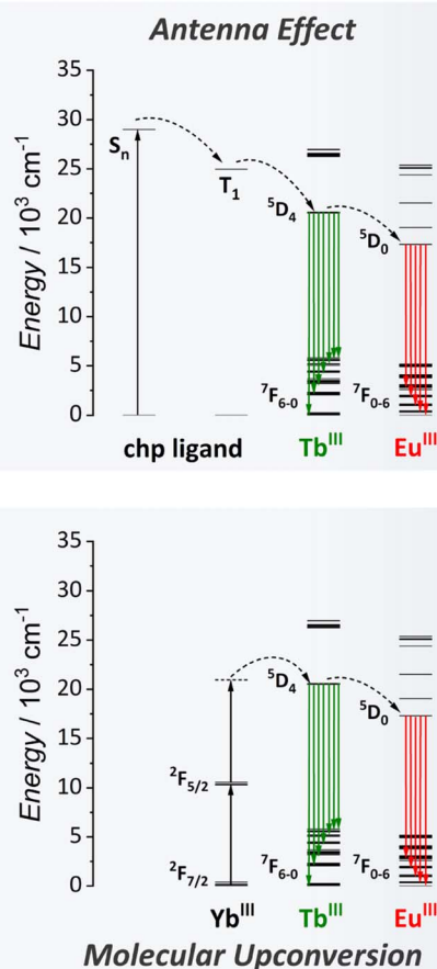
Fig. 7 Metal core structure of the \{Ln_{20}\} MCAs (CCDC number: 2023766) 81 and the energy transfer mechanism for antenna effect and UC emissions. 81,95 Colour code: Dark orange: Ln^{3+} ; grey: carbon; red: oxygen. Hydrogen atoms were omitted in the structure for clarity.
