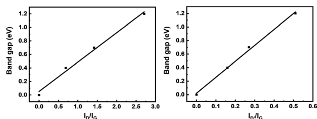
Fig. 4 Band gap of SLG/SLGBr/SLG diodes with different degrees of bromination vs. (a) I_D/I_G and (b) I_D/I_G , respectively.
