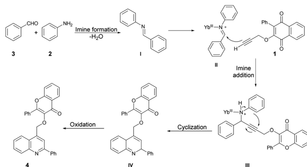
Scheme 3 A proposed mechanism of the one-pot synthesis of quinolin-4-ylmethoxychromen-4-ones catalyzed by YbCl 3 .
