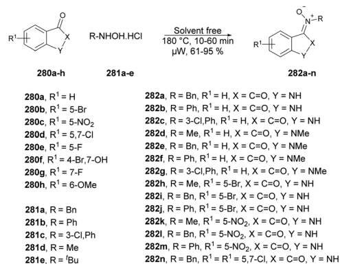
Scheme 99 Synthesis of ketonitrones 282a–n .
