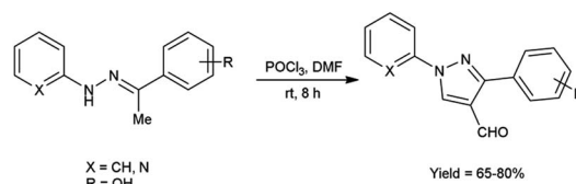
Scheme 10 Synthesis of 3-aryl-4-formyl pyrazoles.
