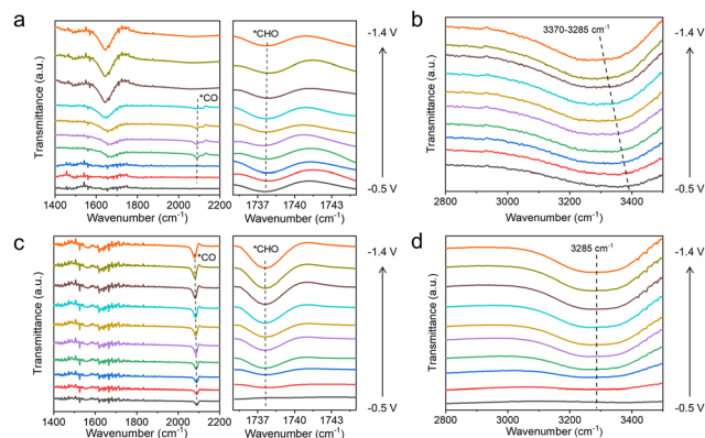
Fig. 4 In situ attenuated total reflection surface-enhanced infrared absorption spectroscopy spectra of (a and b) Cu and (c and d) Cu-3TA catalysts in \text{CO}_2 -saturated 0.1 M \text{KHCO}_3 solution.
