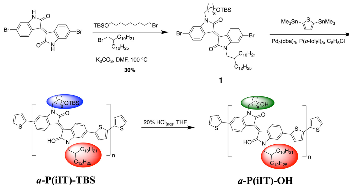
Scheme 1 Synthetic pathway to asymmetric polymer \alpha -P(iIT)-OH.
