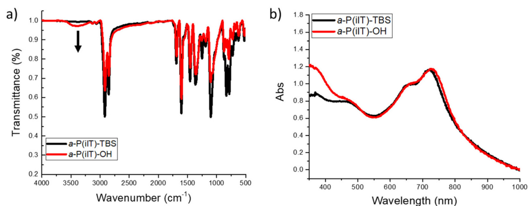
Fig. 1 Fourier-Transform infrared (FTIR) spectra of (a) \alpha -P(iIT)-TBS and \alpha -P(iIT)-OH in the solid-state, and (b) UV-vis spectra of \alpha -P(iIT)-TBS and \alpha -P(iIT)-OH thin films casted on \text{SiO}_2 .
