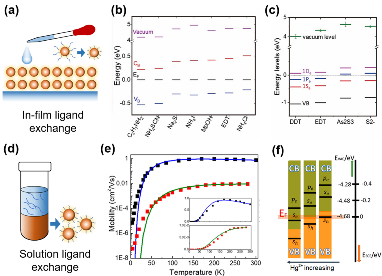
Fig. 7 Ligand exchange and property control of QD films. (a) Schematic of in-film ligand exchange. Various surface ligand induced shifts in the conduction and valence band levels relative to the Fermi level (taken here as 0 eV with reference to all the other energy levels) for (b) HgTe and (c) HgSe QDs with in-film ligand exchange. (b) Is reproduced from ref. 100 with permission from American Chemical Society, copyright 2019. (c) Is reproduced from ref. 78 with permission from American Chemical Society, copyright 2017. (d) Schematic of solution phase ligand exchange. (e) Temperature-dependent FET mobilities of HgSe QDs with hybrid (black) and EDT (red) ligands, solid fitting curves are for Marcus theory of charge hopping. Reproduced from ref. 90 with permission from American Chemical Society, copyright 2020. (f) Controlling doping with HgCl 2 concentration in solution ligand exchange. Reproduced from ref. 101 with permission from American Chemical Society, copyright 2019.
